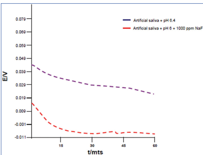
[Table/Fig-7]: Mean galvanic potential when TA coupled with NC.
