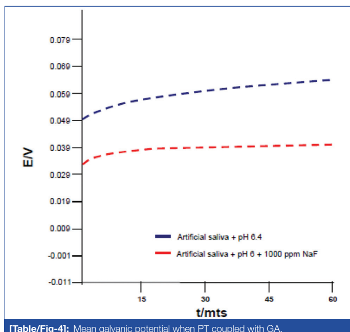
[Table/Fig-4]: Mean galvanic potential when PT coupled with GA.
